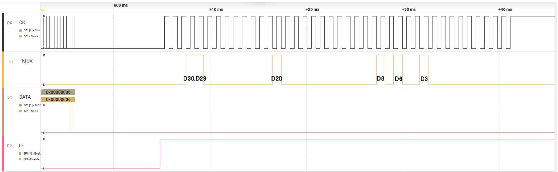
図1. MAX2870 R6 Read back
